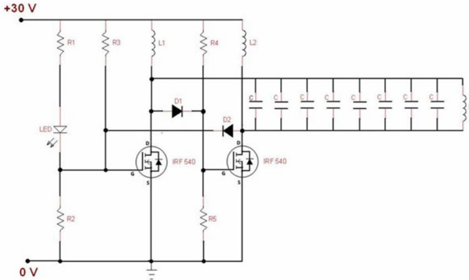
Fig. 2. Transmitter section circuit
