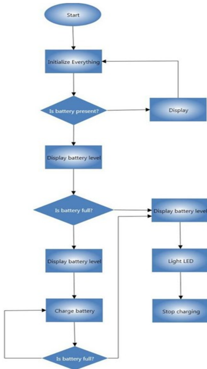
Fig. 10. Code flowchart
