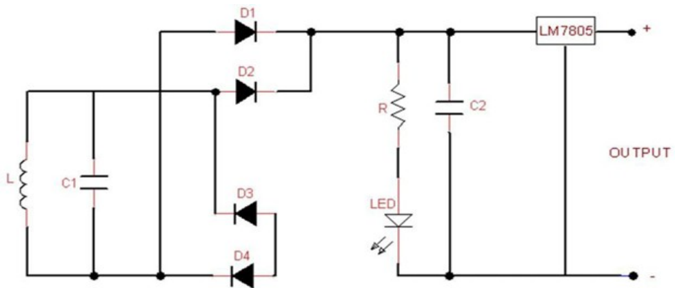
Fig. 3. Receiver circuit
