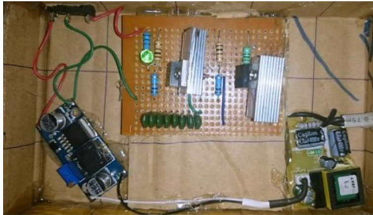
Fig. 11. Components on the Veroboard
