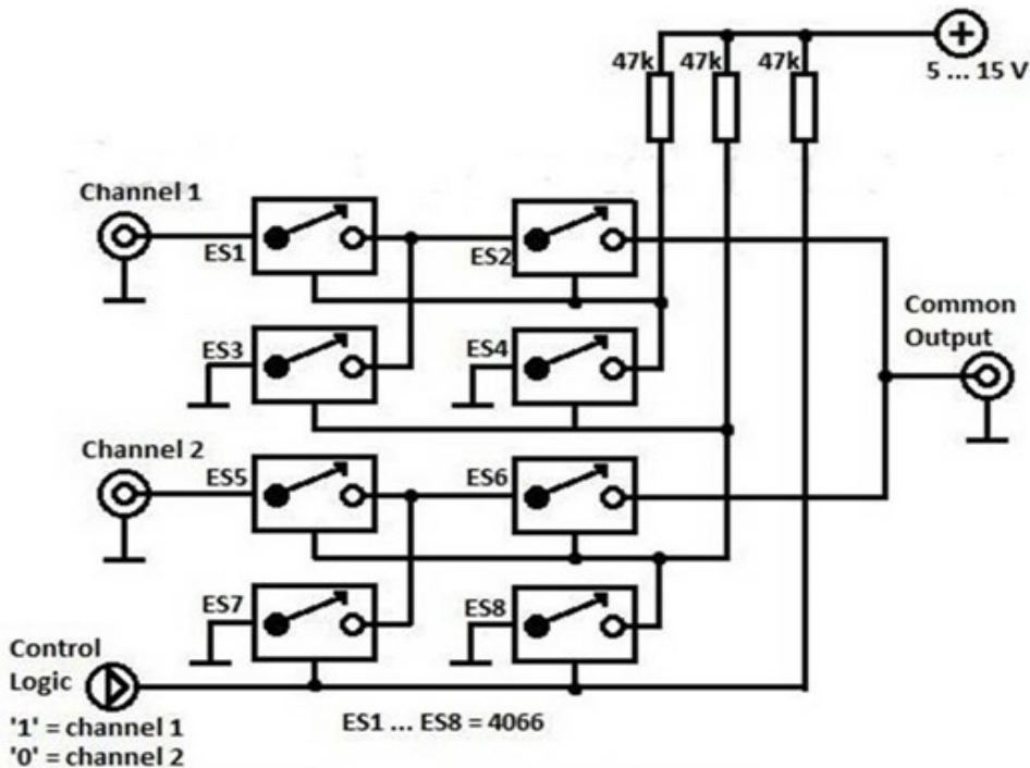
Fig. 9. Multiplexer switch
