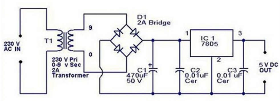
Fig. 4. Power supply
