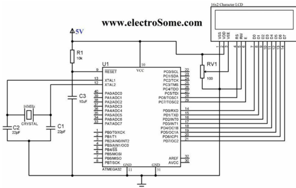
Fig. 8. LCD & Atmega-328 connection
