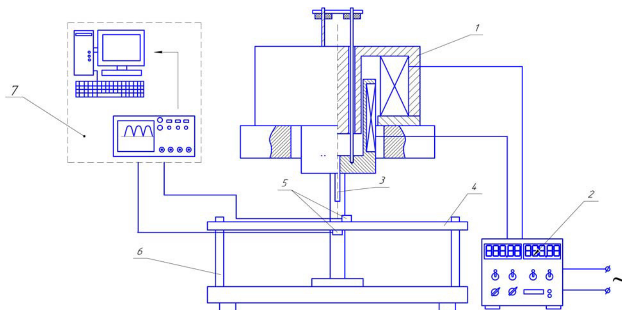
Fig. 1. The scheme of the shock stand
