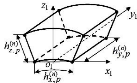
Fig. 3. Single-grid FE V_{n,p}^{(1)}
